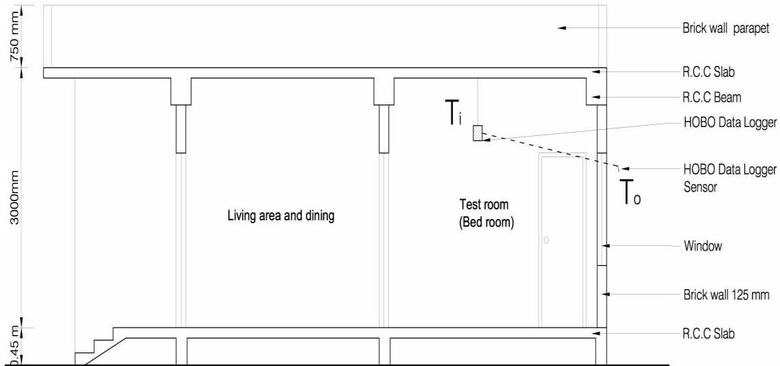
Figure 4. Section of typical contemporary designed house and the position of data logger and sensor.
