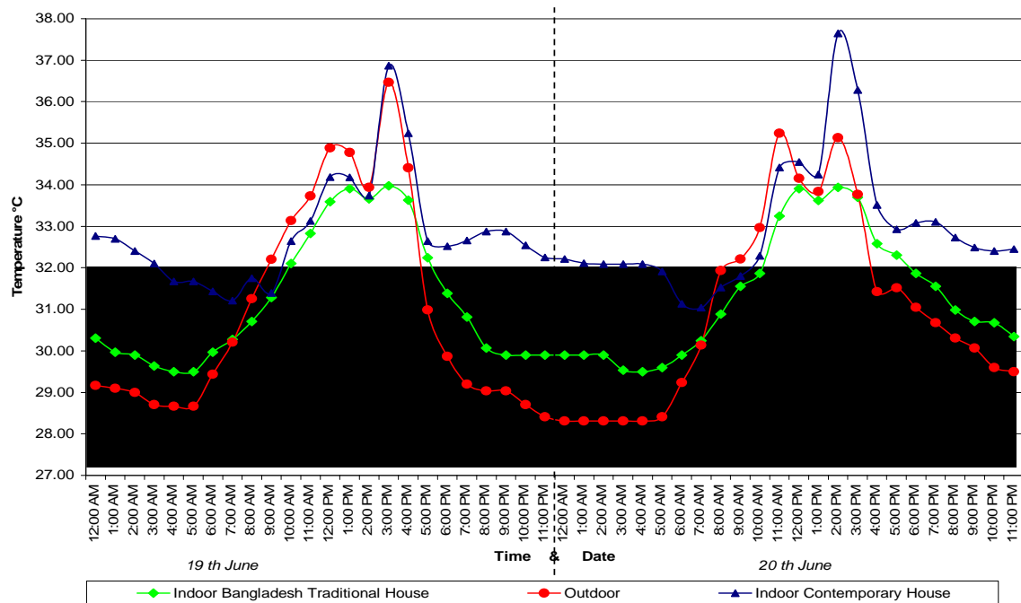
Figure 5: Profile of indoor air temperature of B.T.H (taken from Rumana, (2008)) and C.D.H compare to outdoor air temperature with identified comfort zone.
