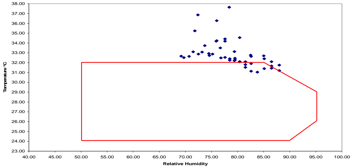
Figure 6. Plotting of the indoor space temperature and the indoor relative Humidity of C.D.H within summer comfort zone.
