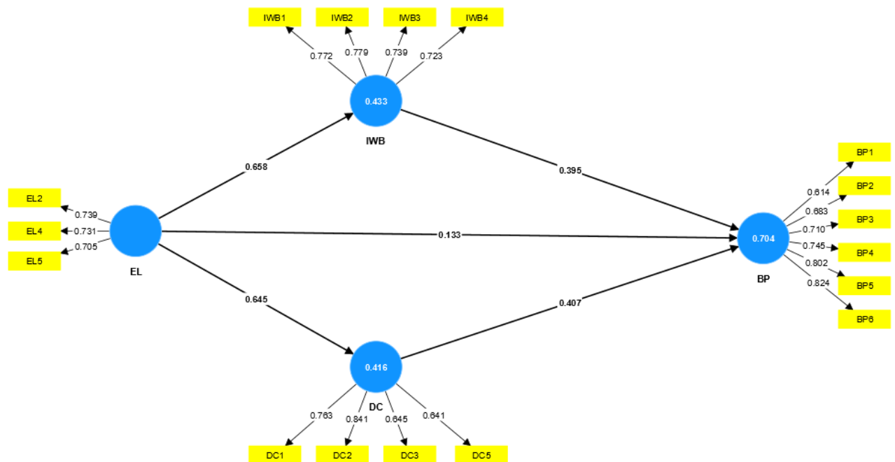
Lampiran 3K: Diagram Jalur PLS Algorithm Ketiga
