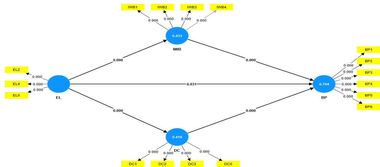
Lampiran 3L: Diagram Jalur Bootstrapping
