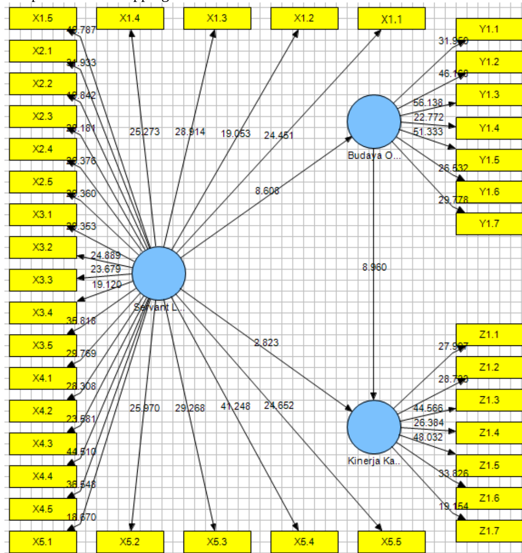
Inner Model T-Statistic
