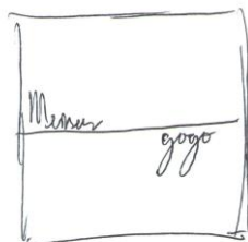
Gambar 4.3. Thumbnail Memo
