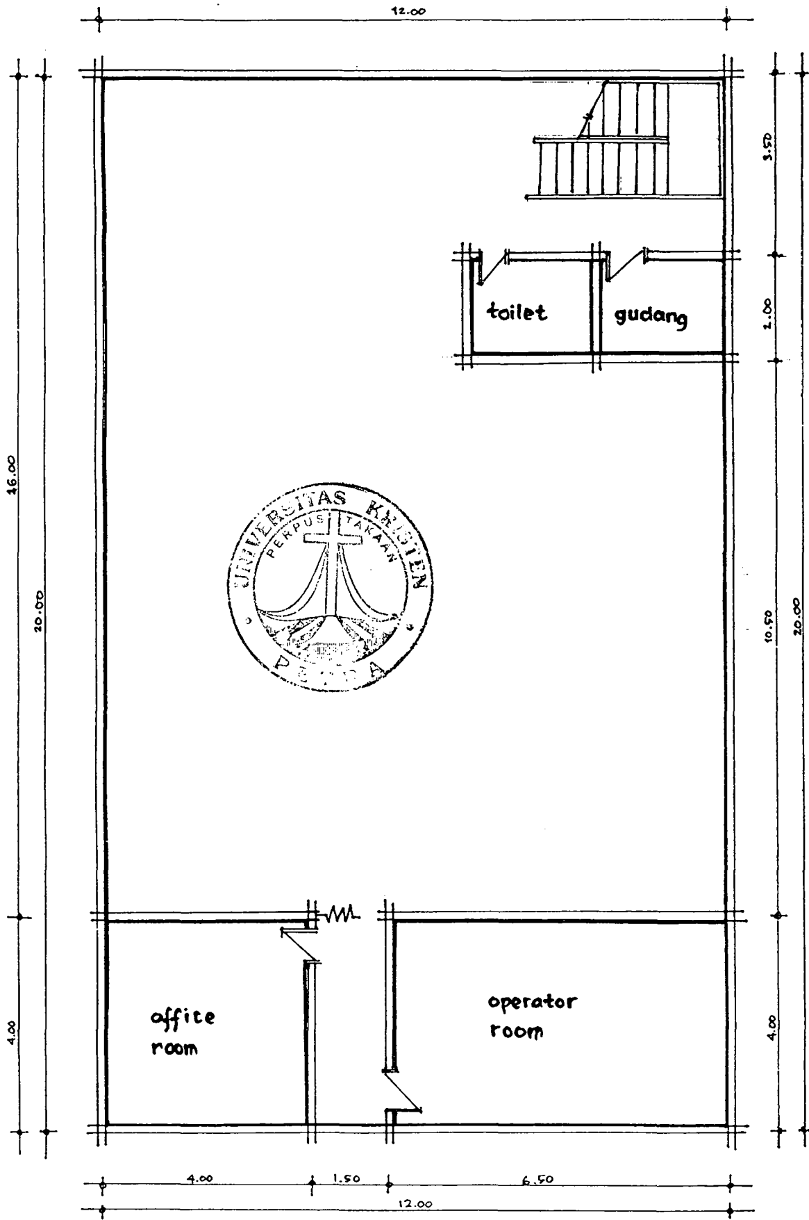
DENAH LT. 3 SKALA 1:100
