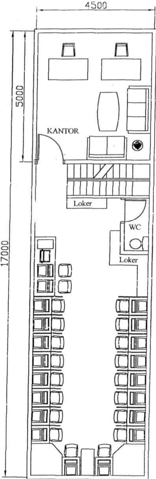
DENAH LANTAI 1
