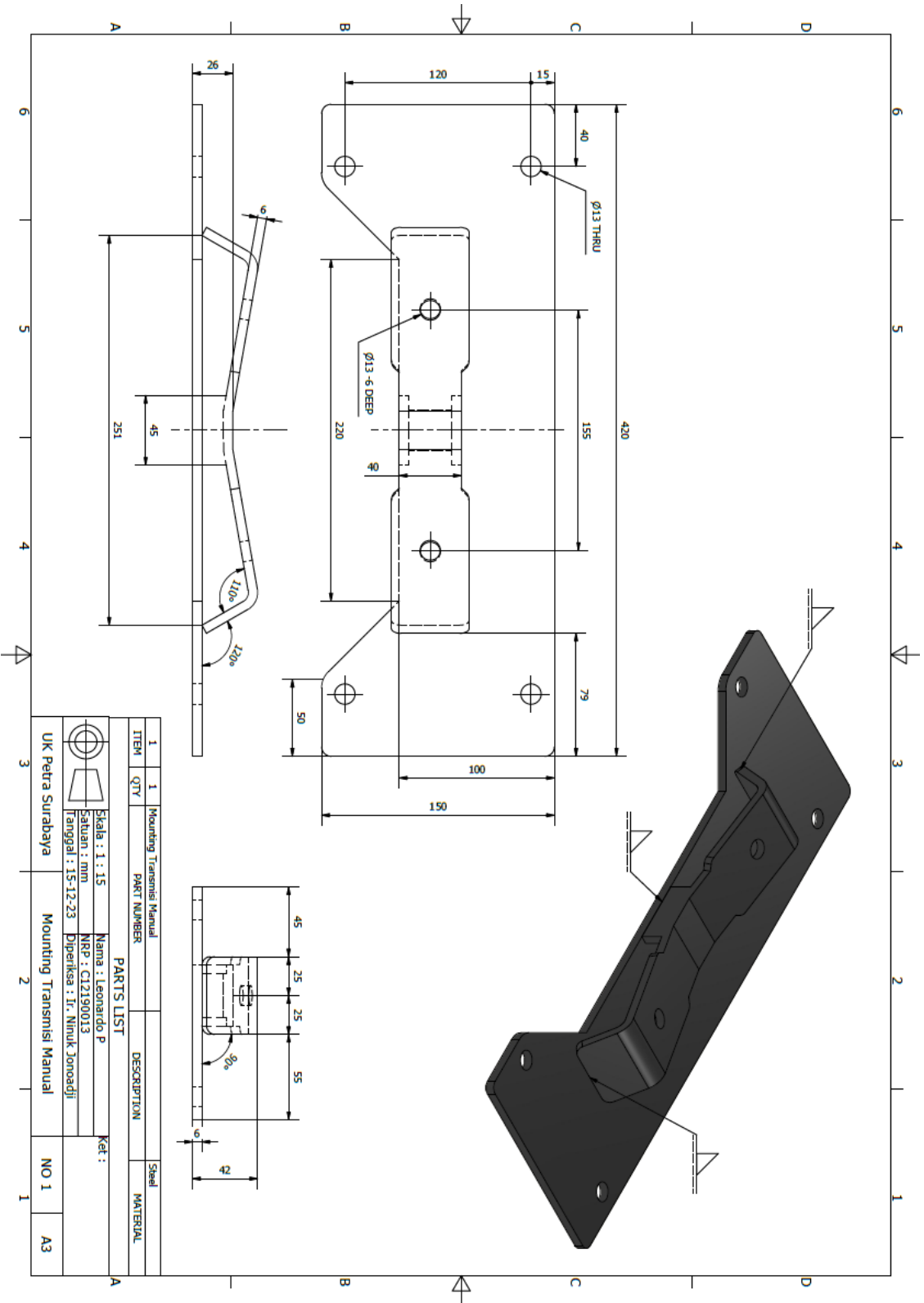
Lampiran 3 : Gambar Teknik Mounting Transmisi
