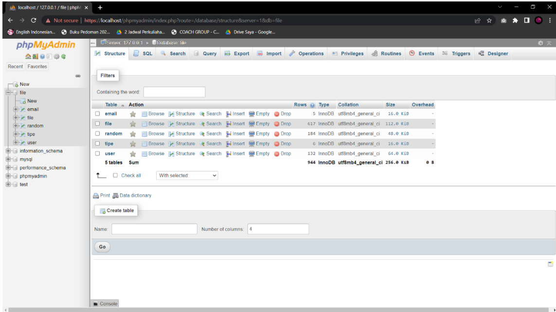
Gambar 4.2 Instalasi phpMyAdmin
