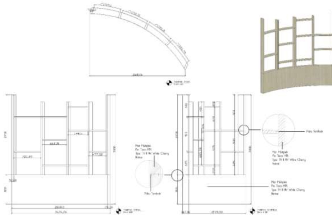
Gambar 7.12 Detail kabinet
