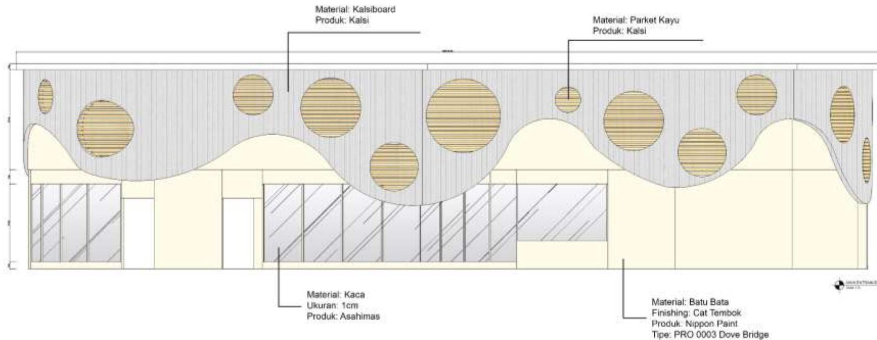
Gambar 7.17. Main entrance
