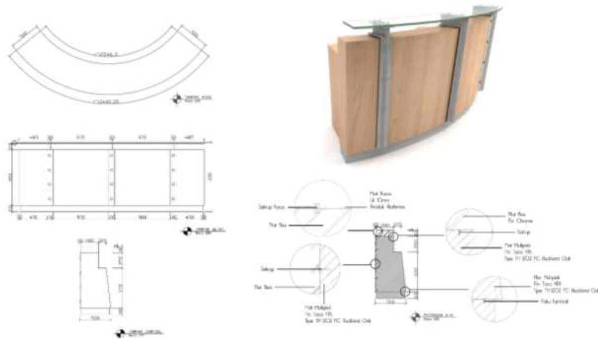
Gambar 7.15. Detail meja resepsionis
