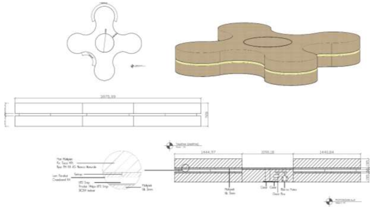
Gambar 7.16. Detail levelling display
