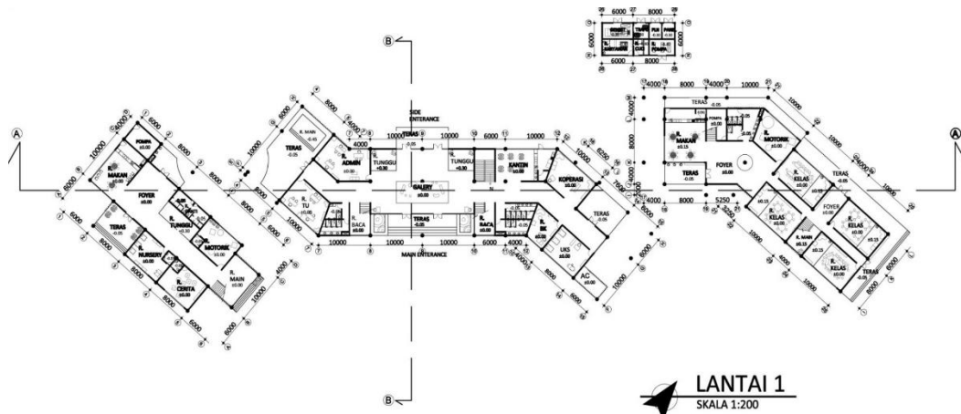
Gambar 3.3. Denah lantai 1
