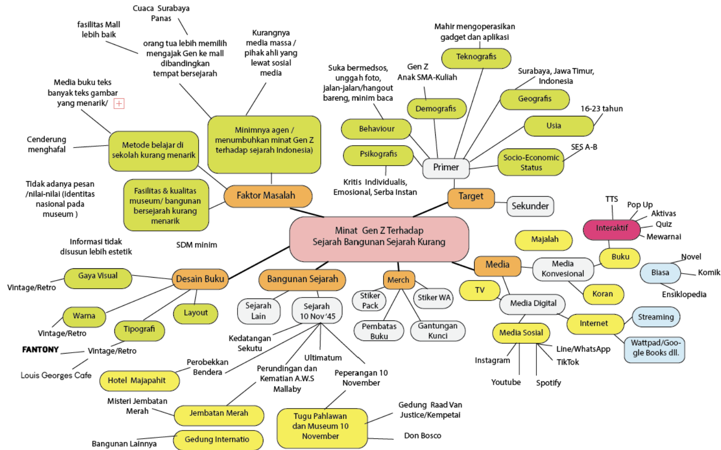
Gambar 3.1. Mindmap
