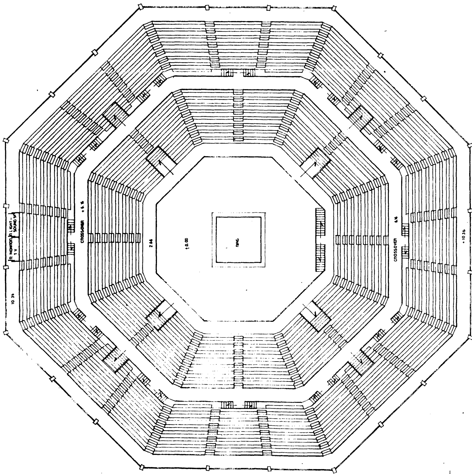
DENAH TRIBUNE SKALA 1:200
